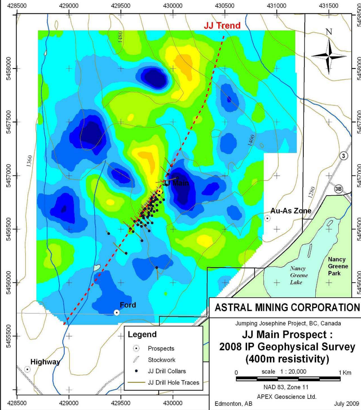
IP Geophysical Survey – Resistivity at 400m
