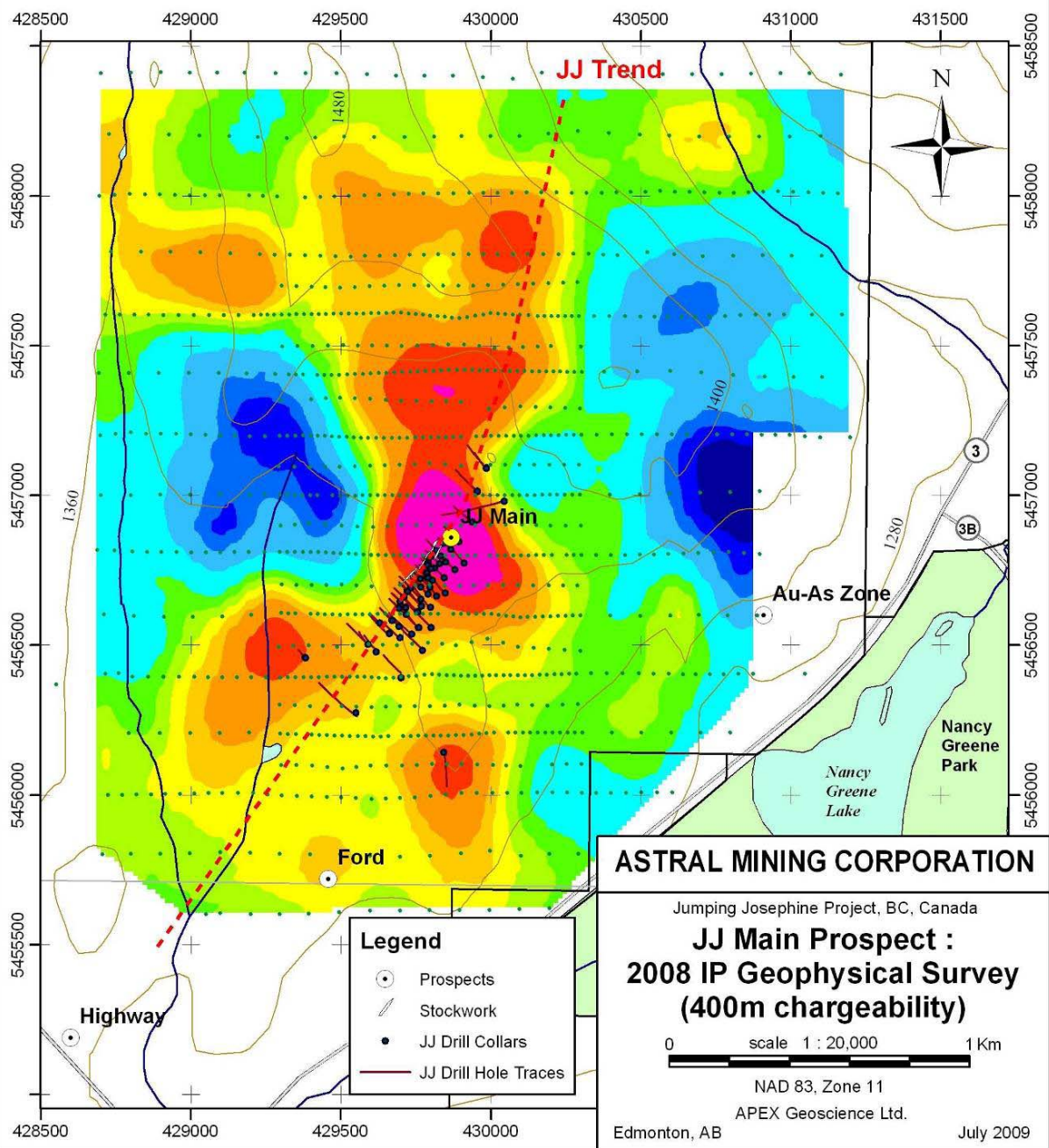
IP Geophysical Survey – Chargeability at 400m
